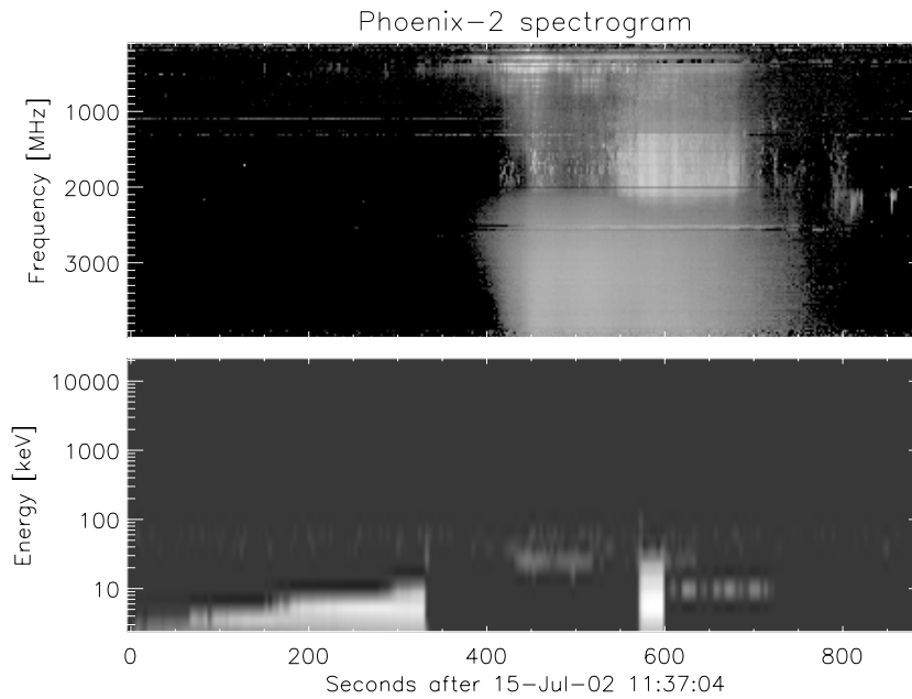
Figure 7. For each event, HEDC has a background-subtracted spectrogram from both RHESSI and Phoenix-2 radio data.
