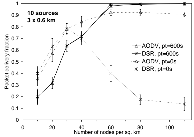
(b) PDF, 3 \times 0.6 \text{ km}^2
