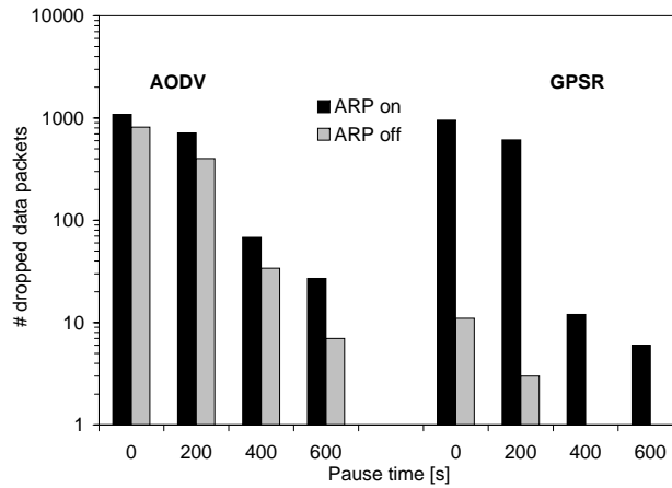
Figure 11: Number of data packets dropped by AODV and GPSR as a function of pause time. “ARP on” – standard ARP is used. “ARP off” – revised ARP version is used. 10 CBR sources.
