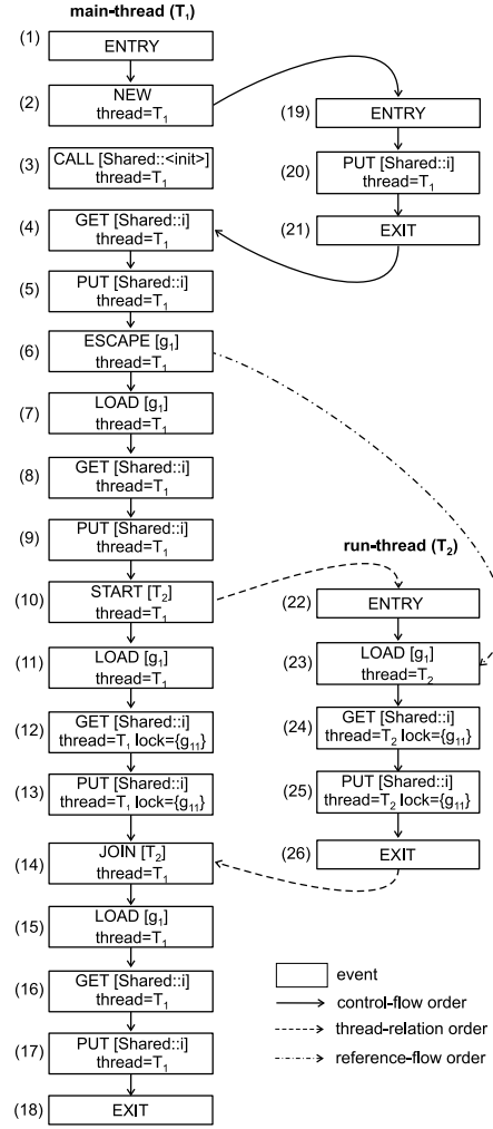
Figure 3: OUG for the abstract object g_{10} of Figure 2.
